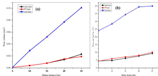
Figure 7: Wear behaviour of FGM casting: (a) Sliding distance versus wear volume and (b) sliding distance versus wear rate
