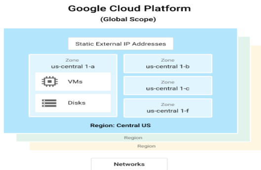
Fig.1: Google Cloud Platform
