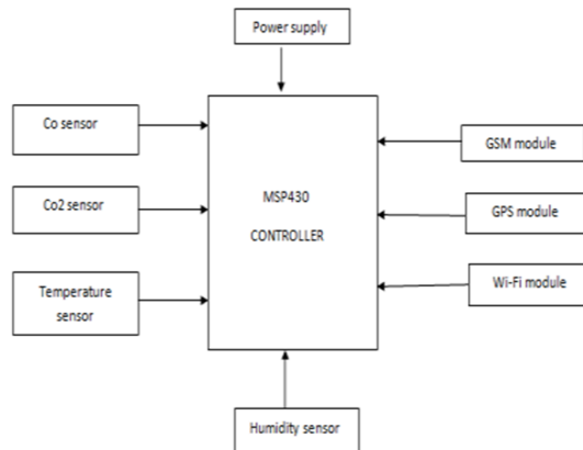
Figure 1 Hardware Description
