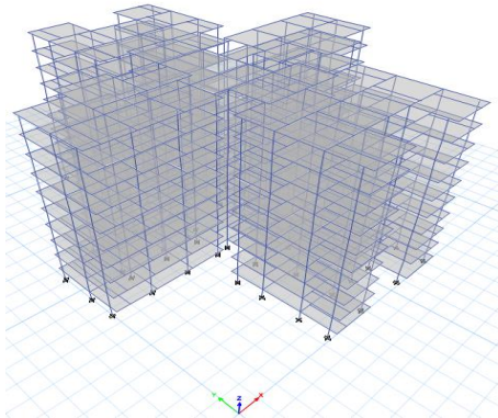
Fig 6: Isometric view of Composite model
