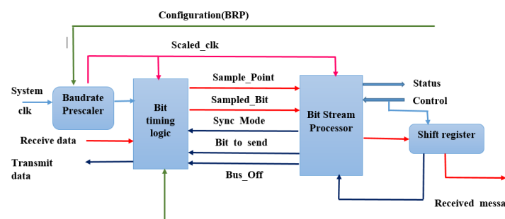
Fig.1 CAN Controller
