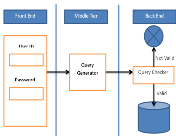
Figure 2: Three tiers proposed Architecture
