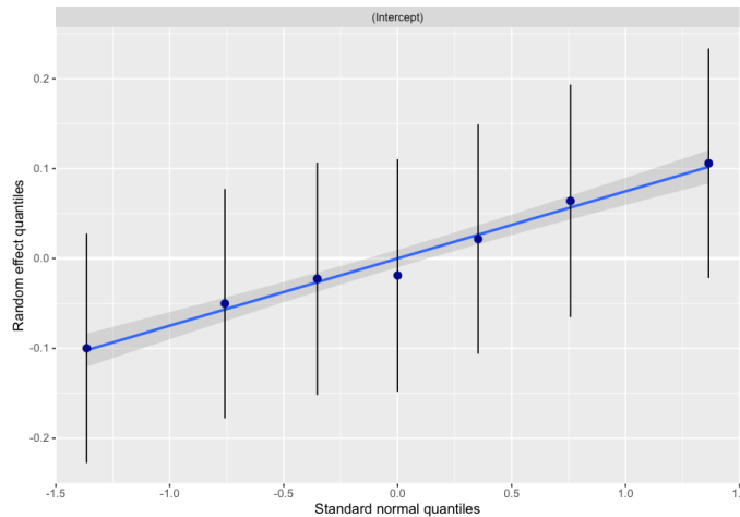
Figure 3: Random effects quantiles with 95% confidence bands
