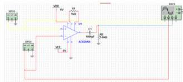
Fig.6. Schematic of AD620 Amplifier circuit
