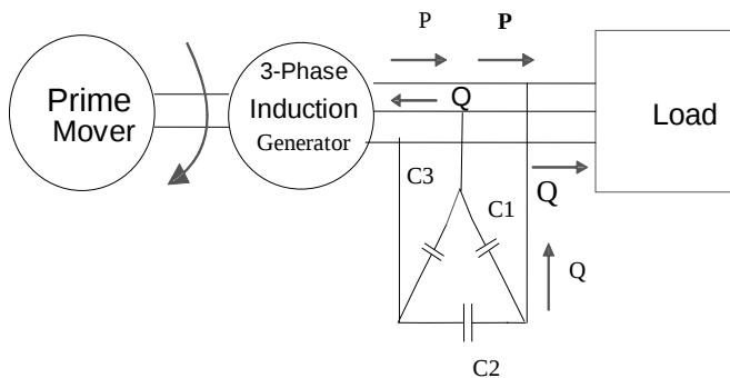
Fig.6. Self Excited Induction Generator
