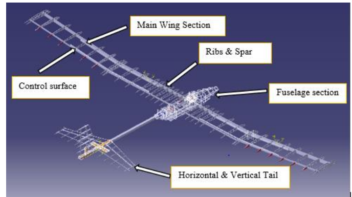
Fig. 12: Finalized Model of UAV
