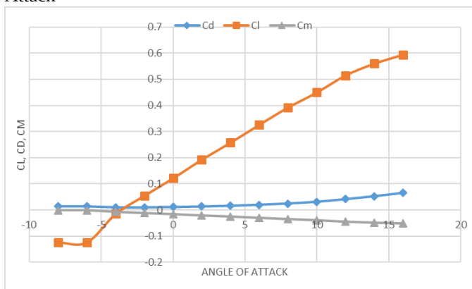
Fig. 20: The graph between lift, drag, moment, and Angle of Attack
