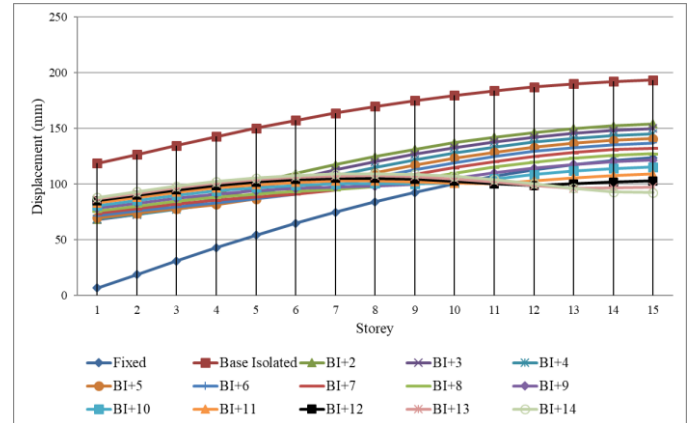
Fig. 5: Storey displacement for RSX load case.
