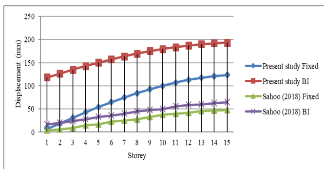
Fig. 9: Comparison of storey displacement.
