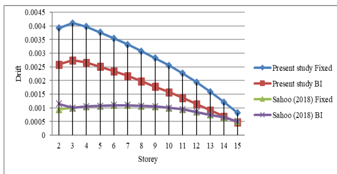
Fig. 10: Comparison of storey drift.
