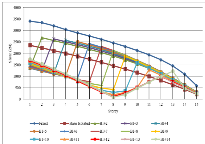
Fig. 8: Storey shear for RSX load case.
