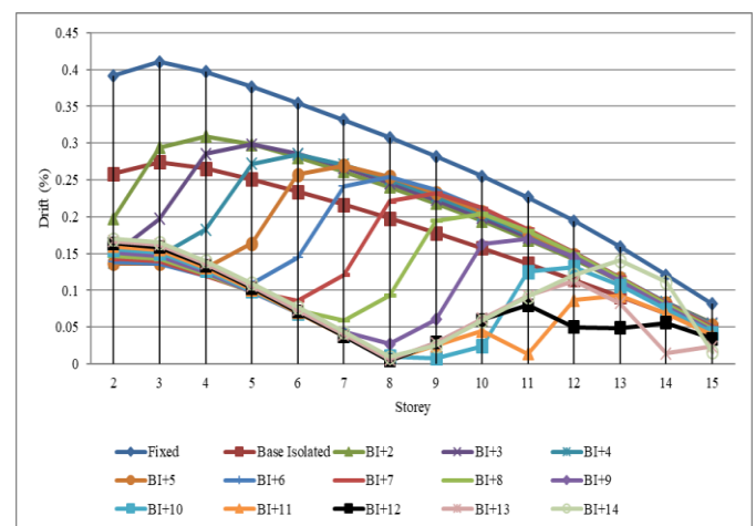
Fig. 6: Storey drift for RSX load case.
