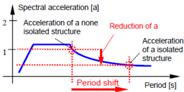
Fig. 4: Period shift due to base isolation (MAURER seismic isolation system with LRB, 2008)
