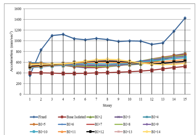
Fig. 7: Storey acceleration for RSX load case.
