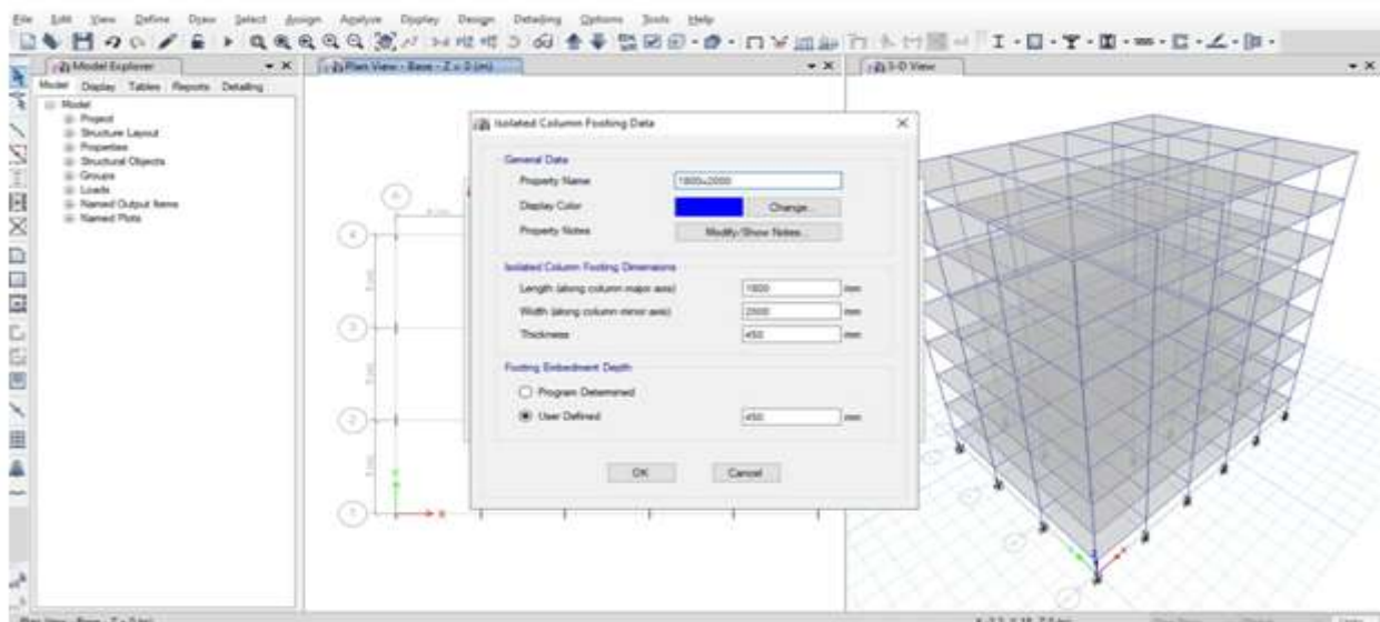
Fig 5.3 Footing Data
