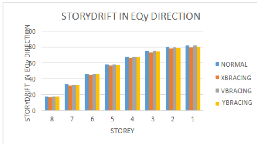
Graph4.4Storey Drift in EQy Direction for Clay
