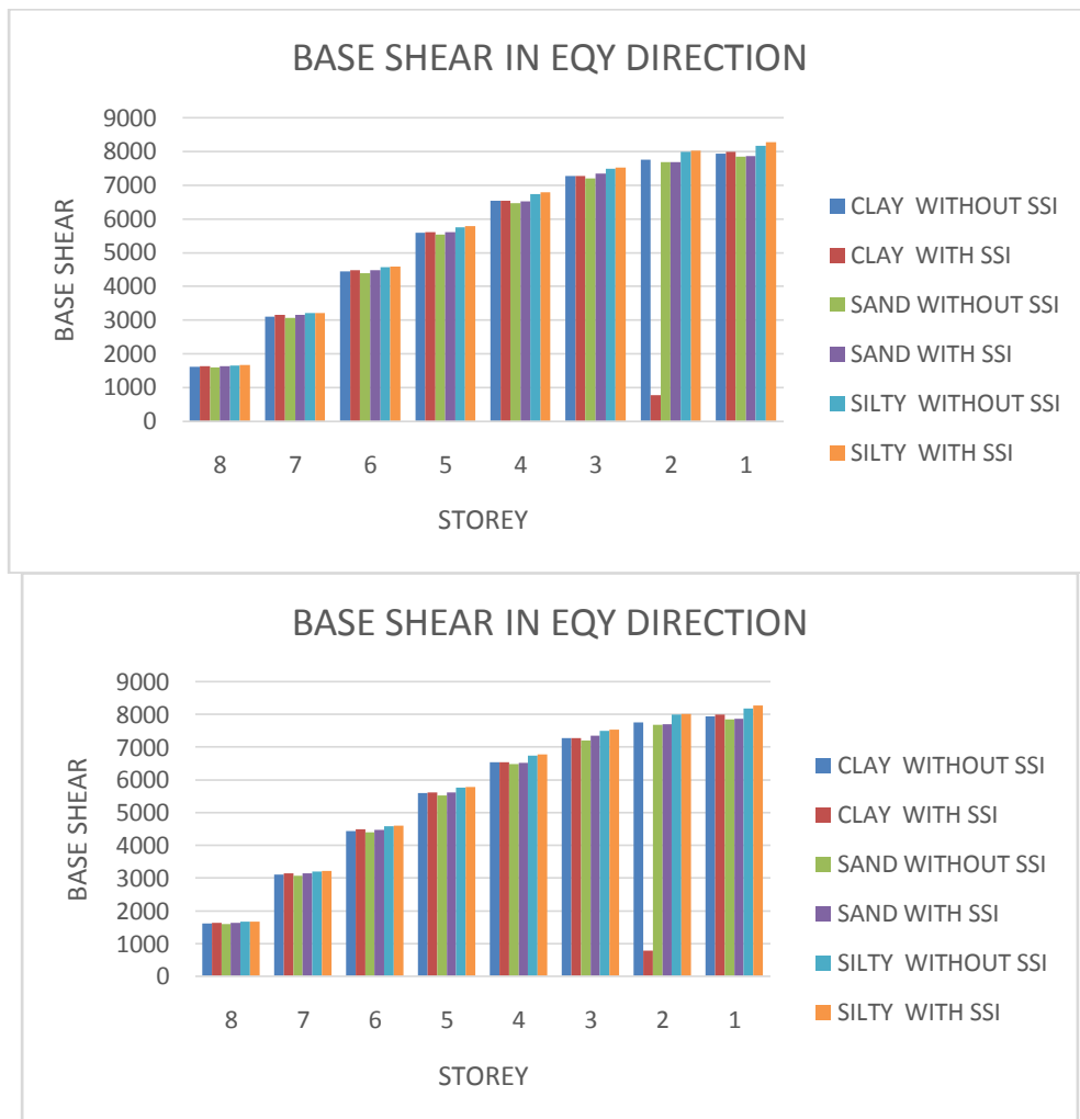
Graph 4.24 Base Shear in EQy direction with and without SSI
