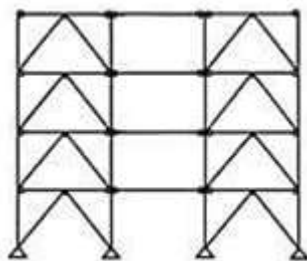
Fig2.5 V-bracing
