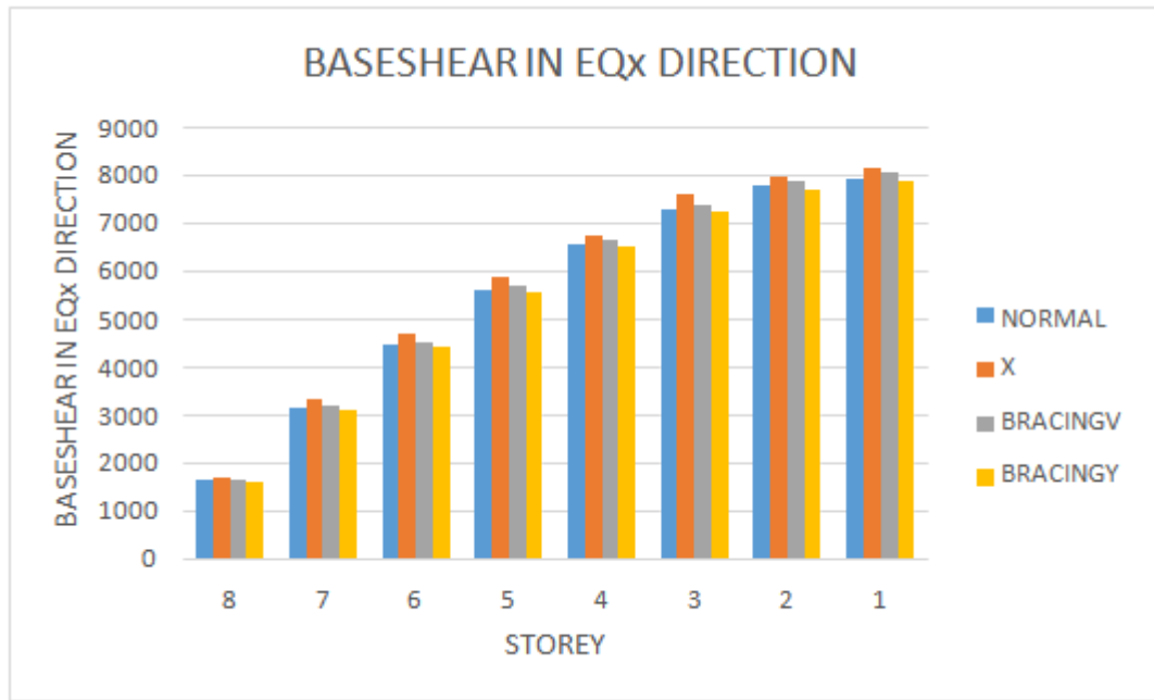
Graph 4.5 Base shear in EQx Direction for Clay
