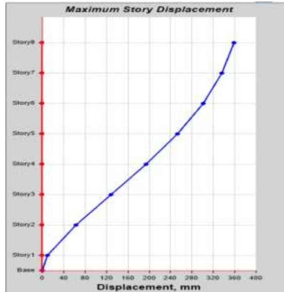
Fig 4.4 Displacement in EQx direction with SSI for clay soil with X bracing
