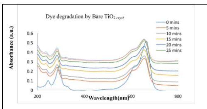
Fig. 10. Dye Degradation by Bare \text{TiO}_{2\text{cryst}}
