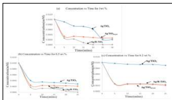
Fig. 12. Photocatalytic efficiency of different silver loaded catalysts.
