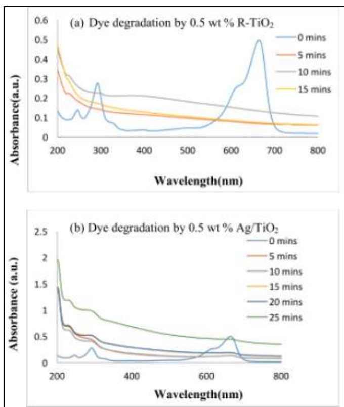
Fig. 11. Degradation of dye by (a) 0.5 wt % \text{Ag/R-TiO}_2 and (b) 0.5 wt % \text{Ag/TiO}_2 in sunlight.
