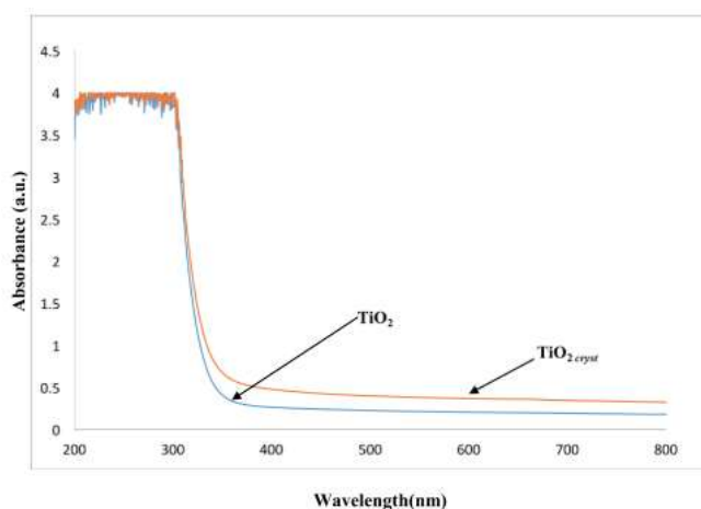
Fig. 4. Absorption spectra of \text{TiO}_2 and \text{TiO}_{2\text{cryst}}
