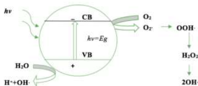
Fig. 1. Generation of oxidative OH radical on TiO 2 surface.
