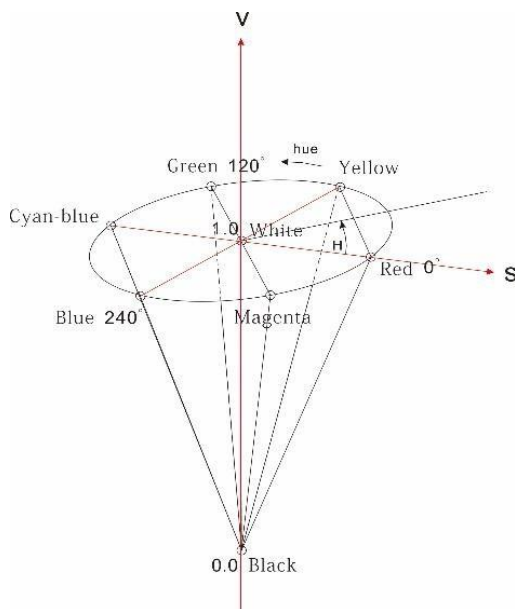
Figure. 1. Three-dimensional HSV hexagonal pyramid.
