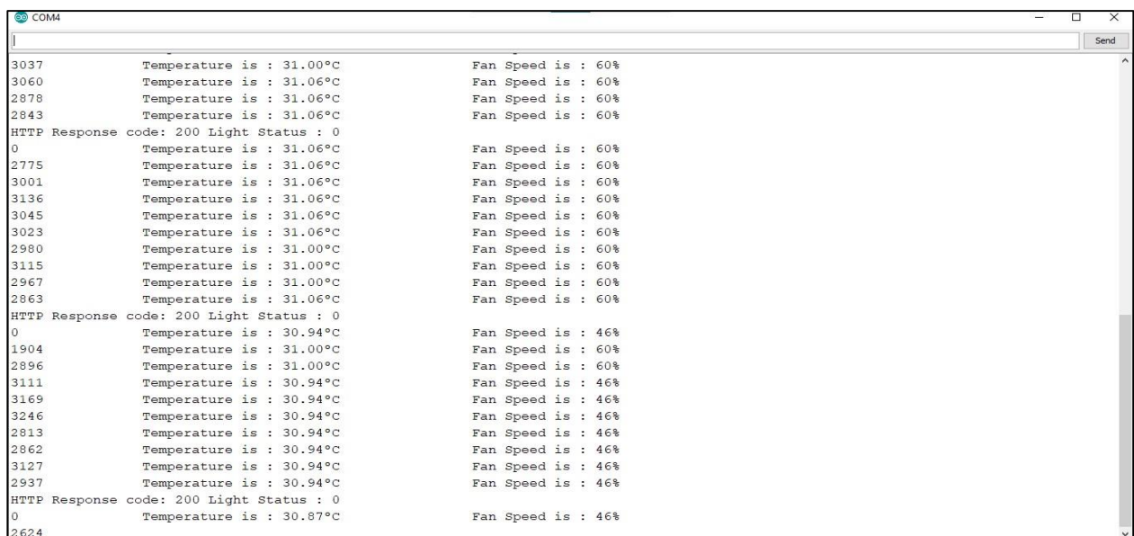
Fig 7: Reading of temperature sensor over serial monitor and change in fan speed depending on temperature sensor value.
