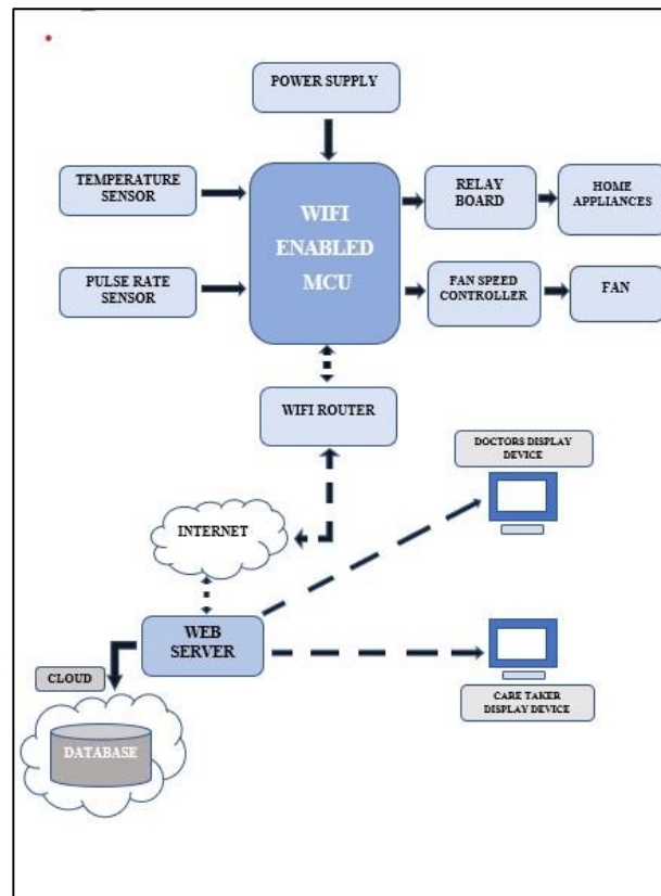
Fig 1: Block Diagram
