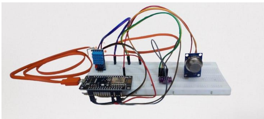
Figure 2: Hardware Design
