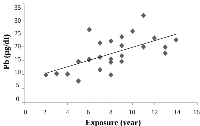
Fig. 3. Correlation coefficient (r) between the blood lead levels (µg/dl) and the duration of exposure (year) in batteries repairing worker group.
