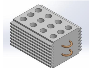
Fig 6.4 3D Diagram of Test Specimen
