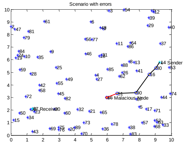
Fig. 5: Scenario 2: With Errors
