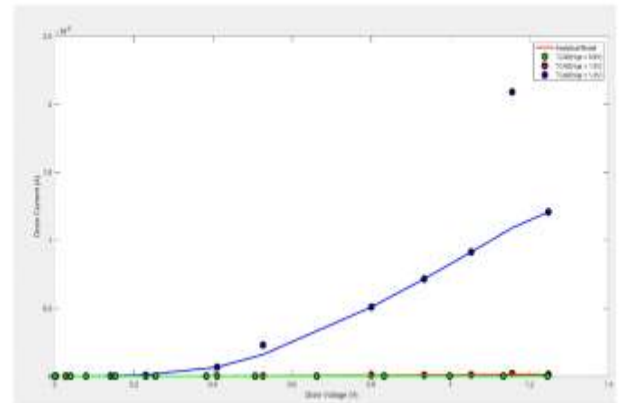
Fig 7. Drain Voltage vs Drain Current
