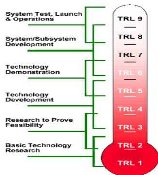
Fig 2: NASA Technology readiness levels 11
