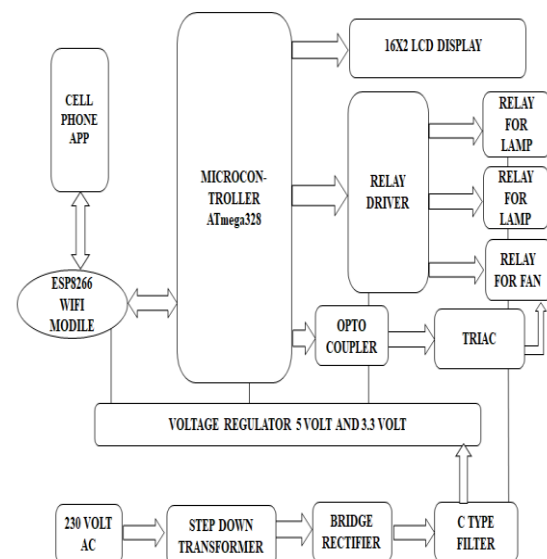
Fig. 1 Block Diagram of IoT based Home Automation
