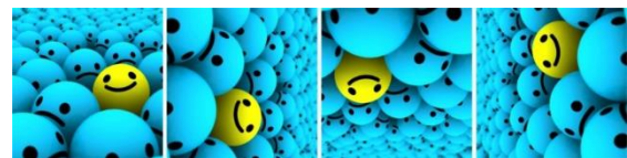
Fig. 2: Data Augmentation
