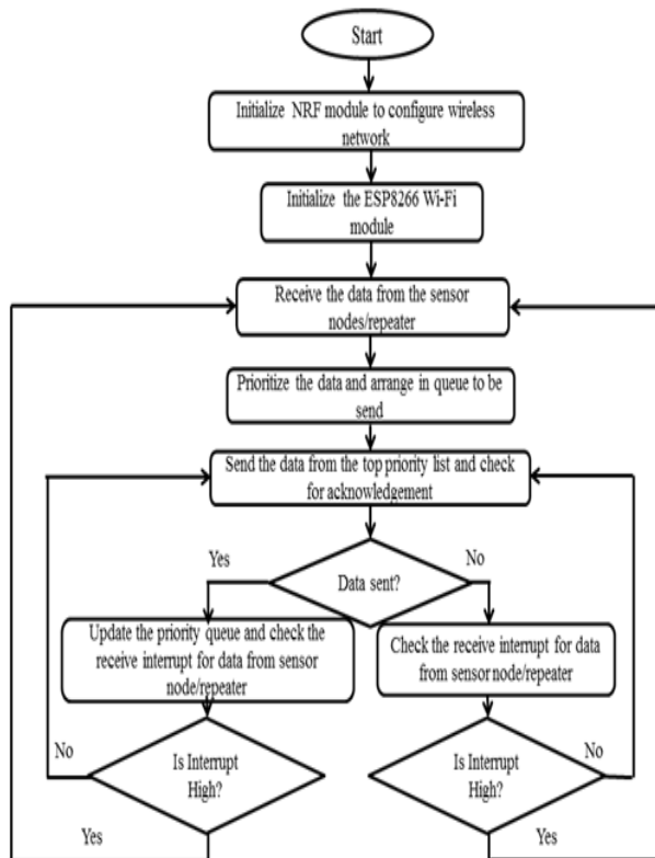
Figure 7: Master Node
