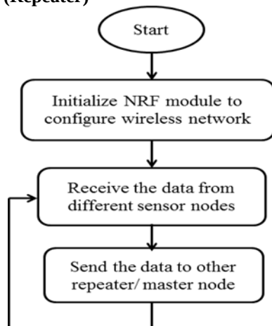
Figure 4. Repeater
