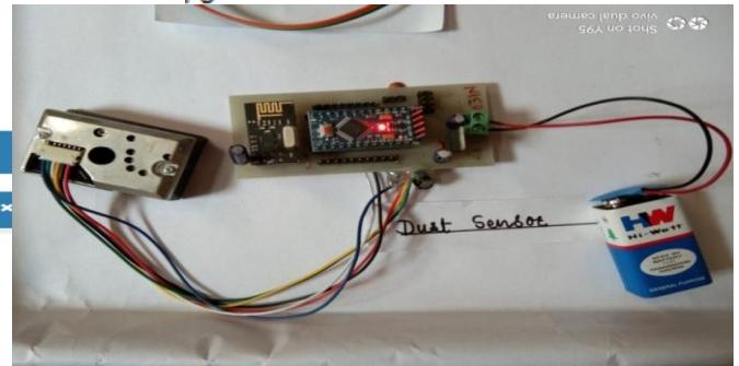
Figure 14: Sensor Node for Dust Sensor
