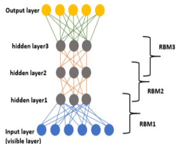
Figure 2: Neural Network Model
