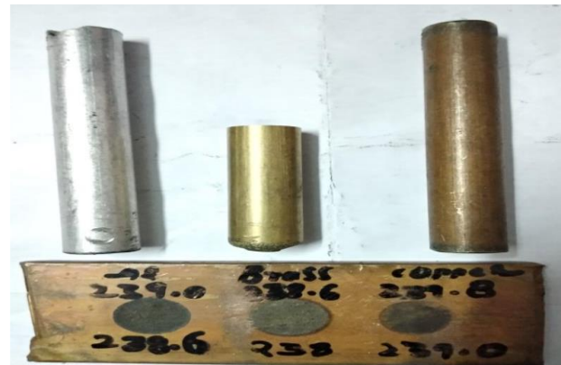
Fig 3. Copper as specimen and copper, brass, aluminium as electrodes
