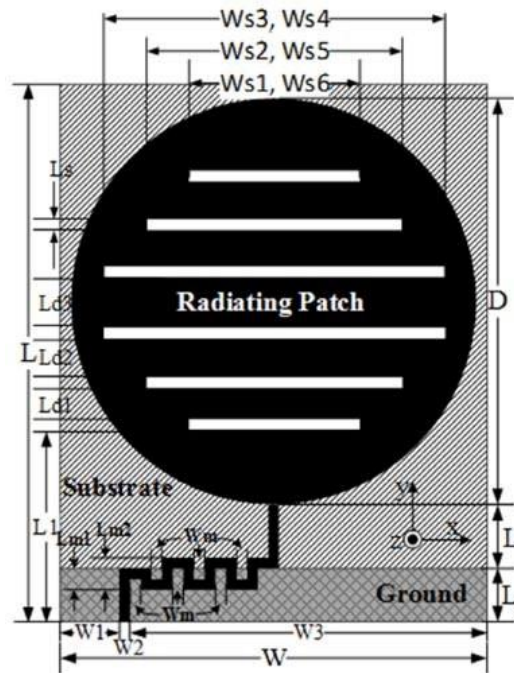
Fig. 2 Circular patch antenna with horizontal slots
