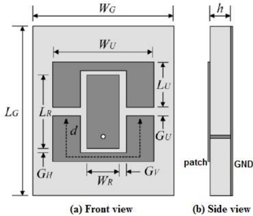
Fig. 3 U-shaped parasitic patch geometry
