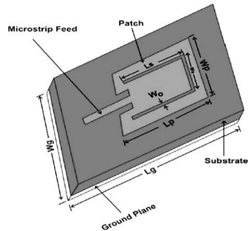
Fig. 1 C-Shaped Slotted Antenna
