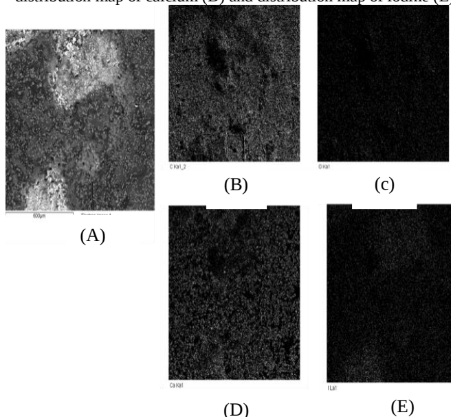
Fig 2. Backscattered electron image of phenanthrene with calcium carbonate exposed to iodine for 4 hr at 21 °C with magnifications 30x (A). Distribution map of carbon (B), distribution map of oxygen (C), distribution map of calcium (D) and distribution map of iodine (E).
