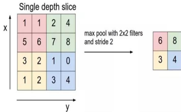
Fig 8: Max Pooling [8]
