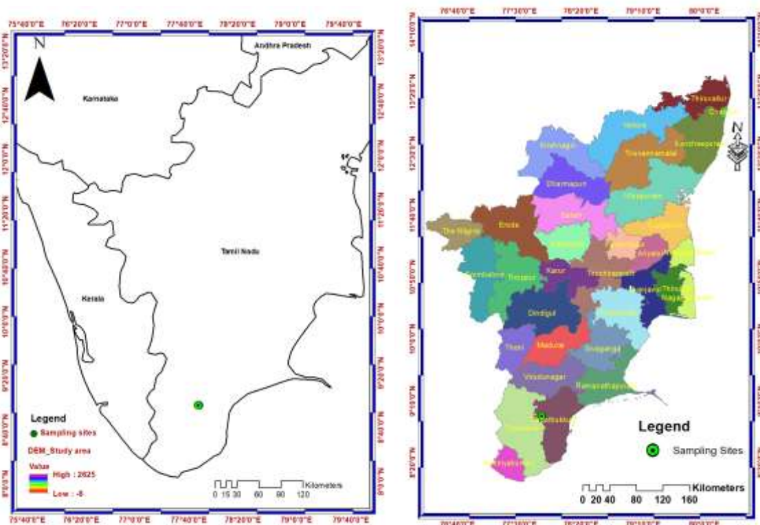
Fig.2 Location Map of the study area, Manur Block
