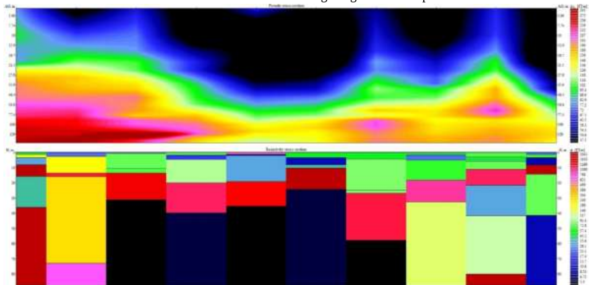
Fig. 6: Resistivity pseudo section and 2D inverse model (Profile 4)
