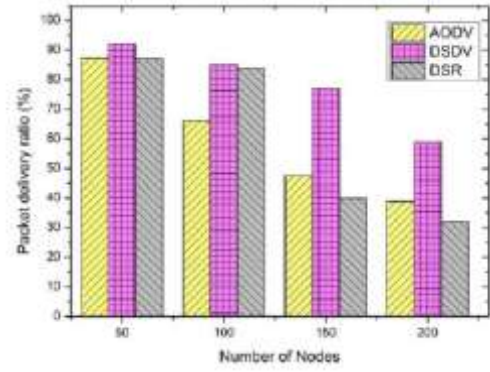
Fig 1. Packet delivery ratio of AODV, DSDV and DSR
