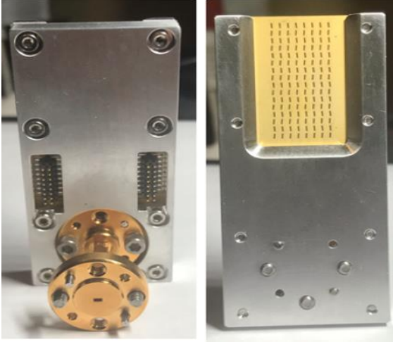
Fig. 3. Nokia RoG 8x16 slot phased array prototype [12]
