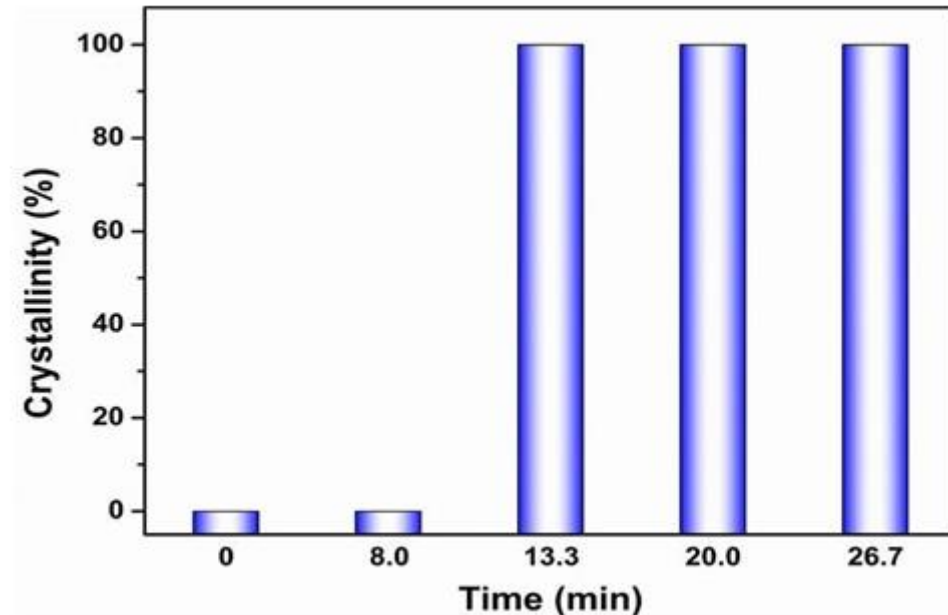
Observing Crystallinity of Zeolite (Na-A) under electron beam irradiation for 0, 8.0,13.3, 20.0, and 26.7 minutes
