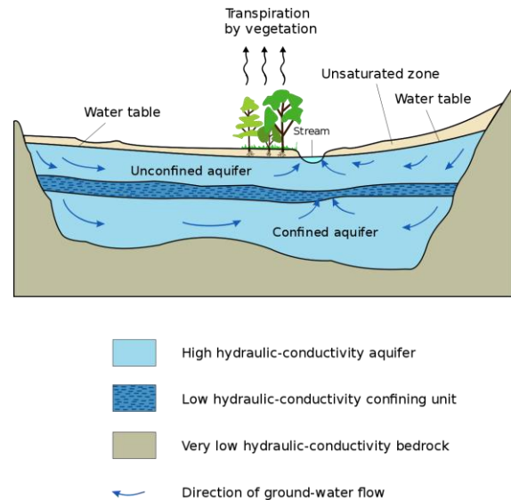
Fig. 1. Aquifer
