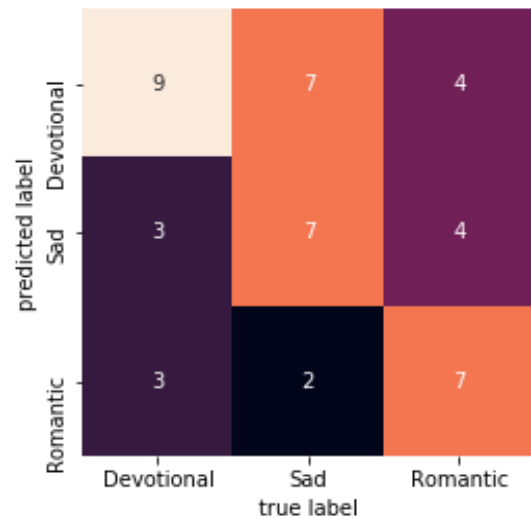
Fig 10. Confusion matrix for Parallel CNN RNN model
