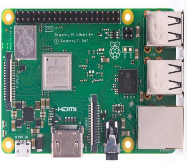
Fig 3: The Raspberry Pi board
