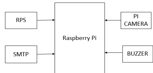
Fig 2: Block Diagram of smart surveillance system
