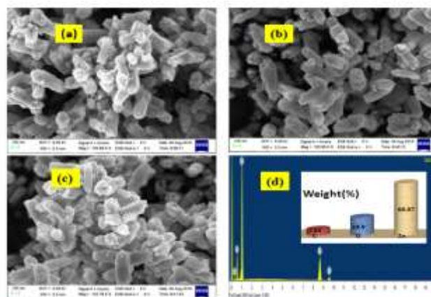
5(a-c) FE SEM images of ZnO nano rods synthesized using aqueous leaf extract of Ficus Hispidula L. and (d) EDS spectrum of ZnO nano rods.
