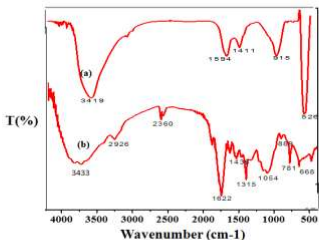
Fig.3(a) FTIR spectrum of Ficus Hispidula L. leaf powder and (b) FTIR spectrum of synthesized ZnO nano rods
