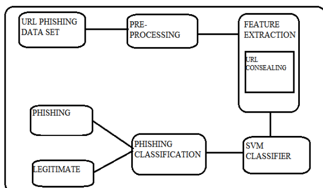
Fig 3.2 : Block diagram for proposed system
