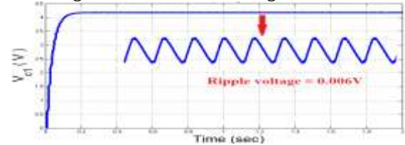
Fig. 15. Voltage across Capacitor C_1
