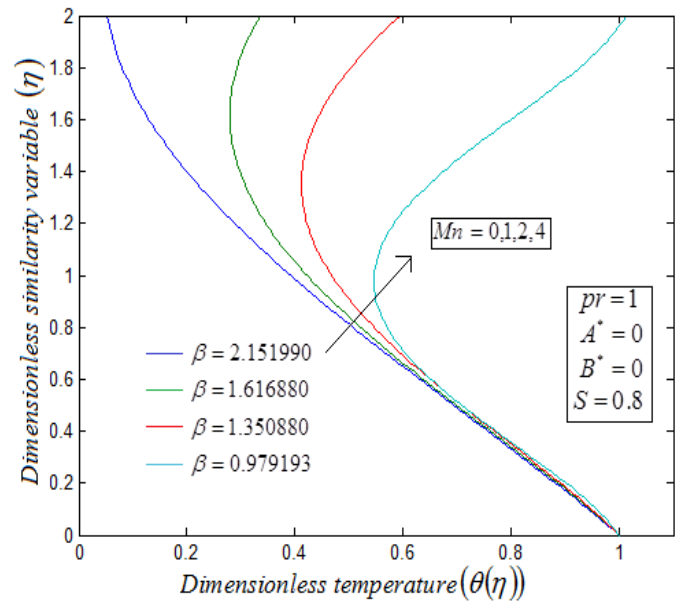
Fig.4: Dimensionless temperature( \theta(\eta) )versus dimensionless similarity variable( \eta ). The curves are plotted for various values of the dimensionless film thickness( \beta ), magnetic parameter( Mn )and some fixed value of the other parameter S, pr, A^*, B^* using the eqn.(26) when h = 0.3025 .
