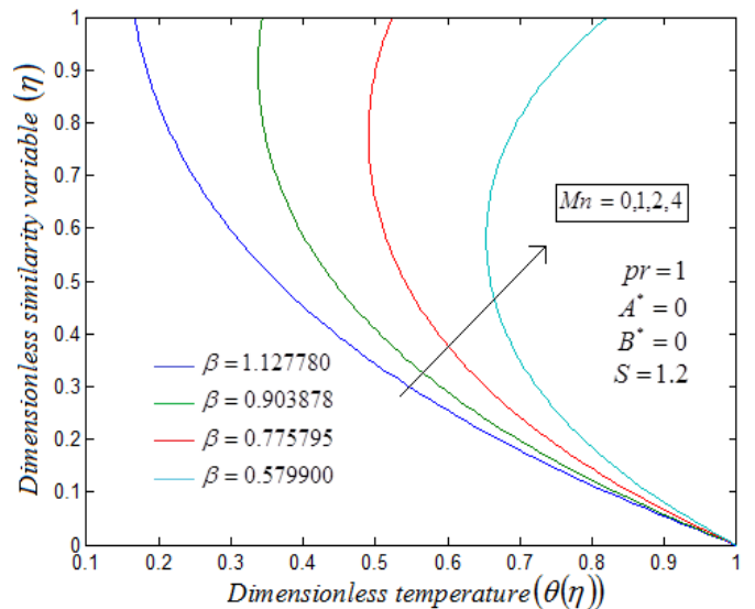
Fig.5: Dimensionless temperature( \theta(\eta) )versus dimensionless similarity variable( \eta ). The curves are plotted for various values of the dimensionless film thickness( \beta ), magnetic parameter( Mn )and some fixed value of the other parameter S, pr, A^*, B^* using the eqn.(26) when h = 0.3025 .
