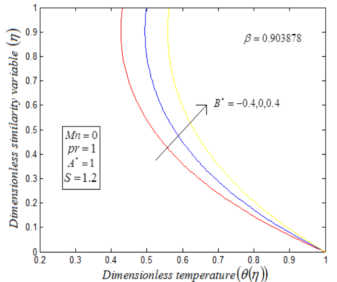
Fig.9: Dimensionless temperature ( \theta(\eta) ) versus dimensionless similarity variable ( \eta ). The curves are plotted for various values of the coefficient of temperature ( B^* ) and some fixed value of the other parameter S, pr, A^*, Mn, \beta using the eqn.(26) when h = -0.8033 .
