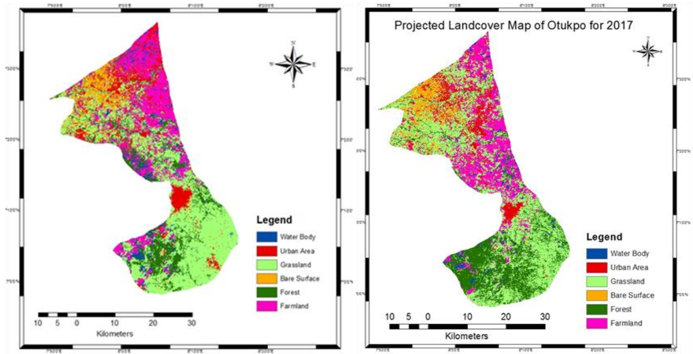
Figure 8: Land cover maps of Otukpo for 2017 (Actual, left and predicted, right) Source: Author's fieldwork, 2018
