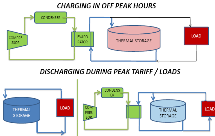
Fig.4. Simplified Thermal Energy Storage for Air Conditioning
