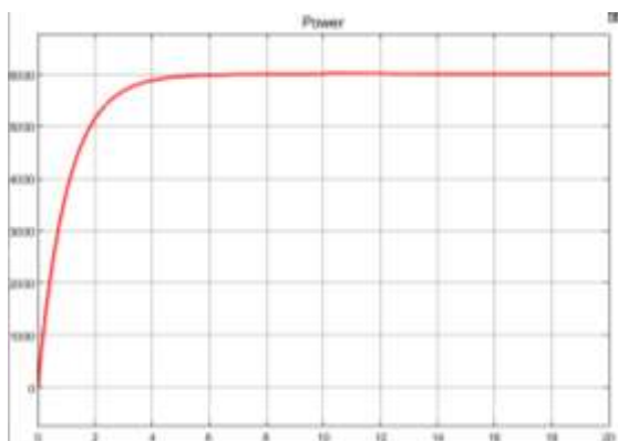
Fig 19: Time-Power Characteristics of PEMFC
