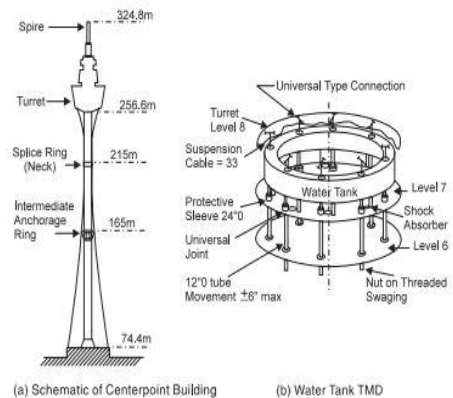
Fig. 7. Water Tank TMD at Centerpoint Tower Sydney Australia
