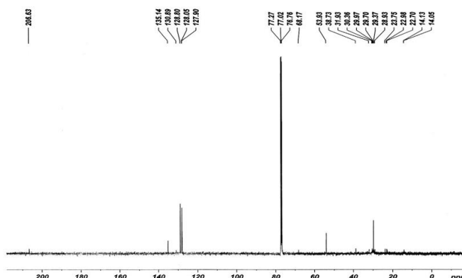
Fig.4 ^{13}\text{C} NMR spectra of [\text{Pb}(\text{pndtc})_2]
