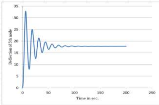
Chart -14: Displacement of the 5th node of the chimney using 1.5% TMD at 5th and 1st node The maximum deflection of the 5 th node is investigated by using 1.5% Multiple TMD on different nodes and results are observed.
