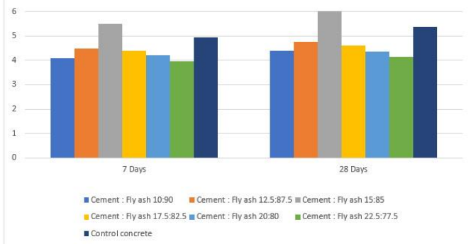
Fig 6. Comparison of Flexural strength of fly ash aggregate concrete and control concrete vs Number of days of curing
