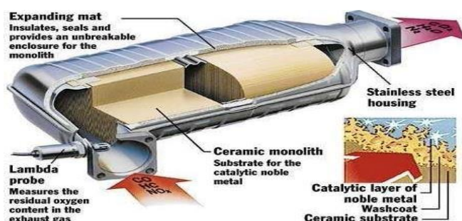
Fig. 1 Cross-sectional view of catalytic convertor
