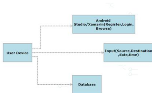
Figure 9 Component Diagram
