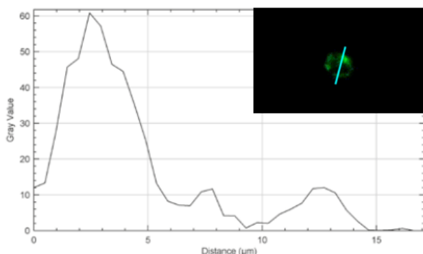
Fig. 5. ImageJ software
